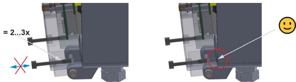
Fig. 23-4 Screw plugs: secured / collision avoided
