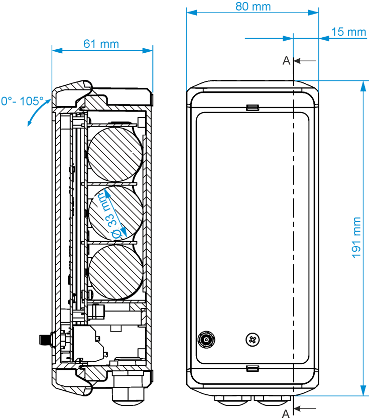
Fig. 17-4 Enclosure for non-Ex device versions
