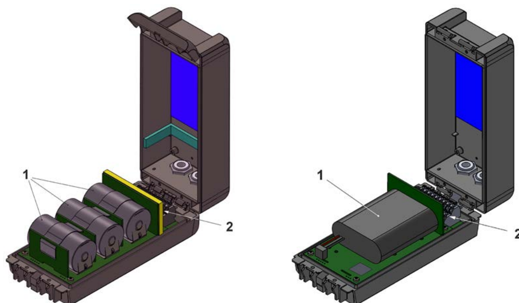
Fig. 3-1 Power supply by batteries / rechargeable batteries
